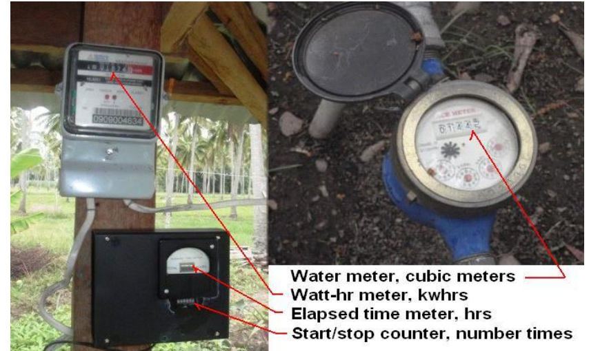
Instrumentation and metering equipment to track electric and water usage for better management control.
